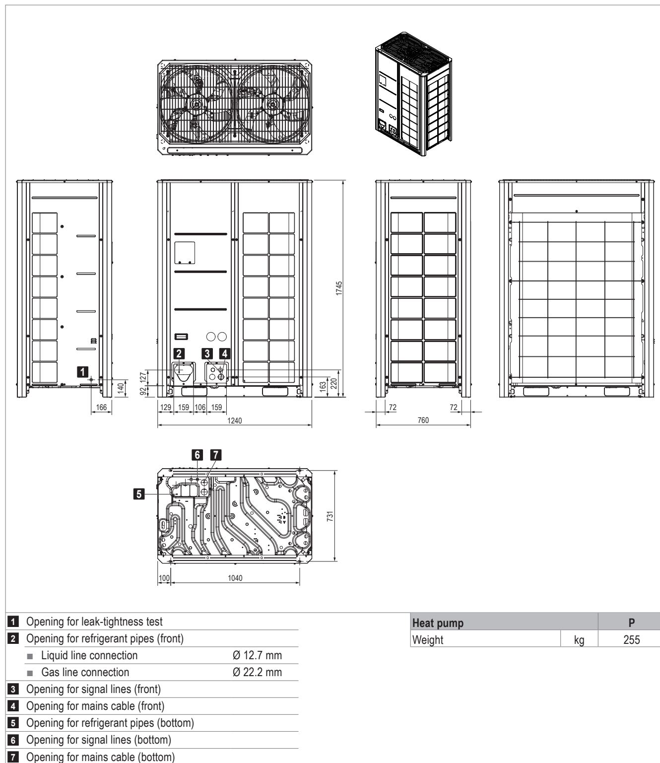
Fig. B8: Heat pump P dimensions and weights
