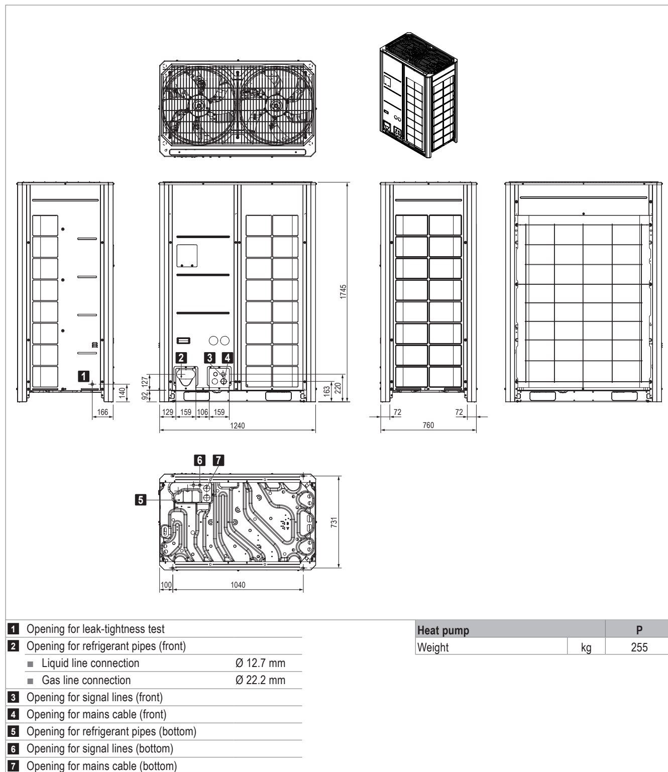
Fig. C8: Heat pump P dimensions and weights
