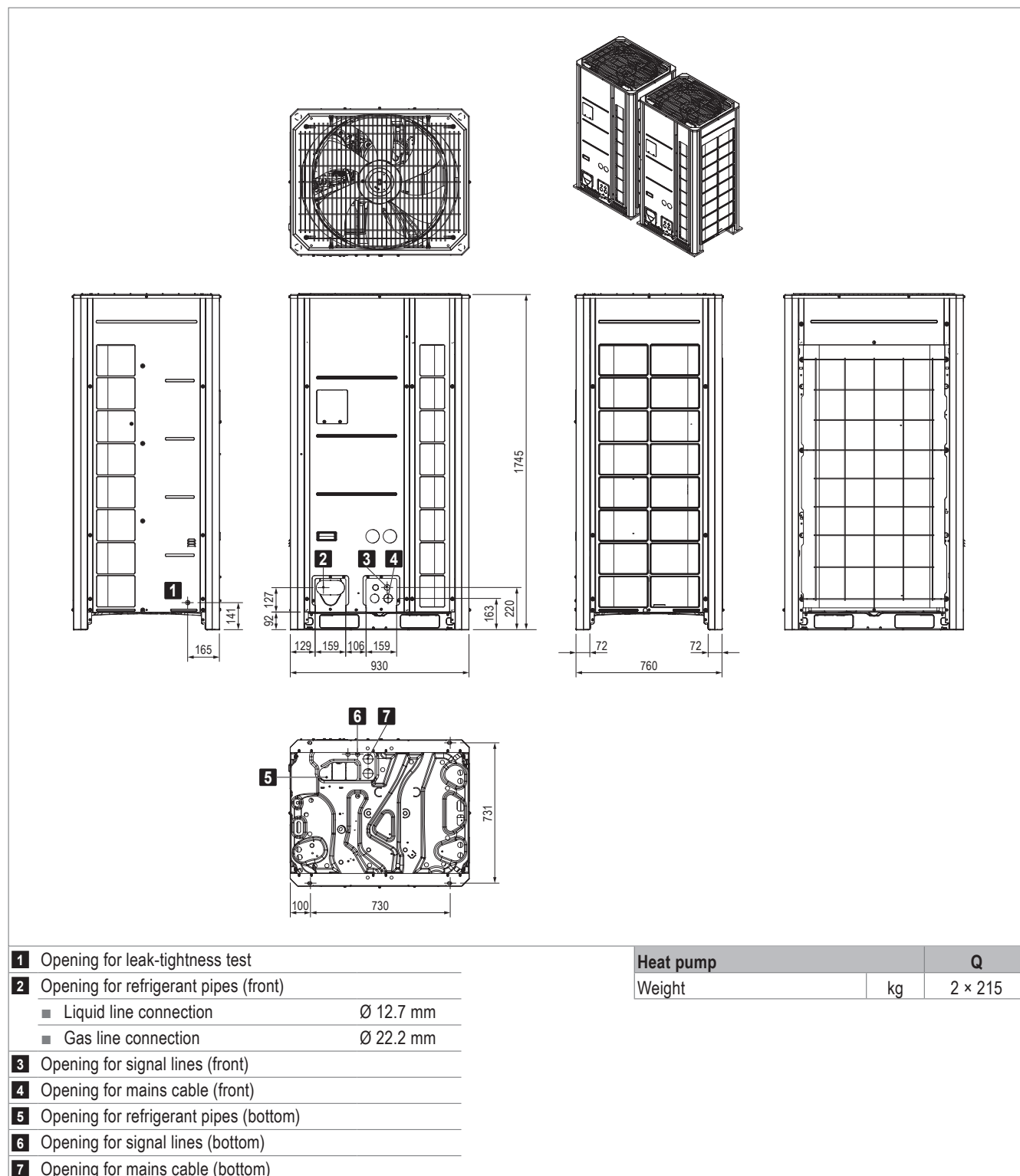
Fig. B10: Heat pump Q dimensions and weights
