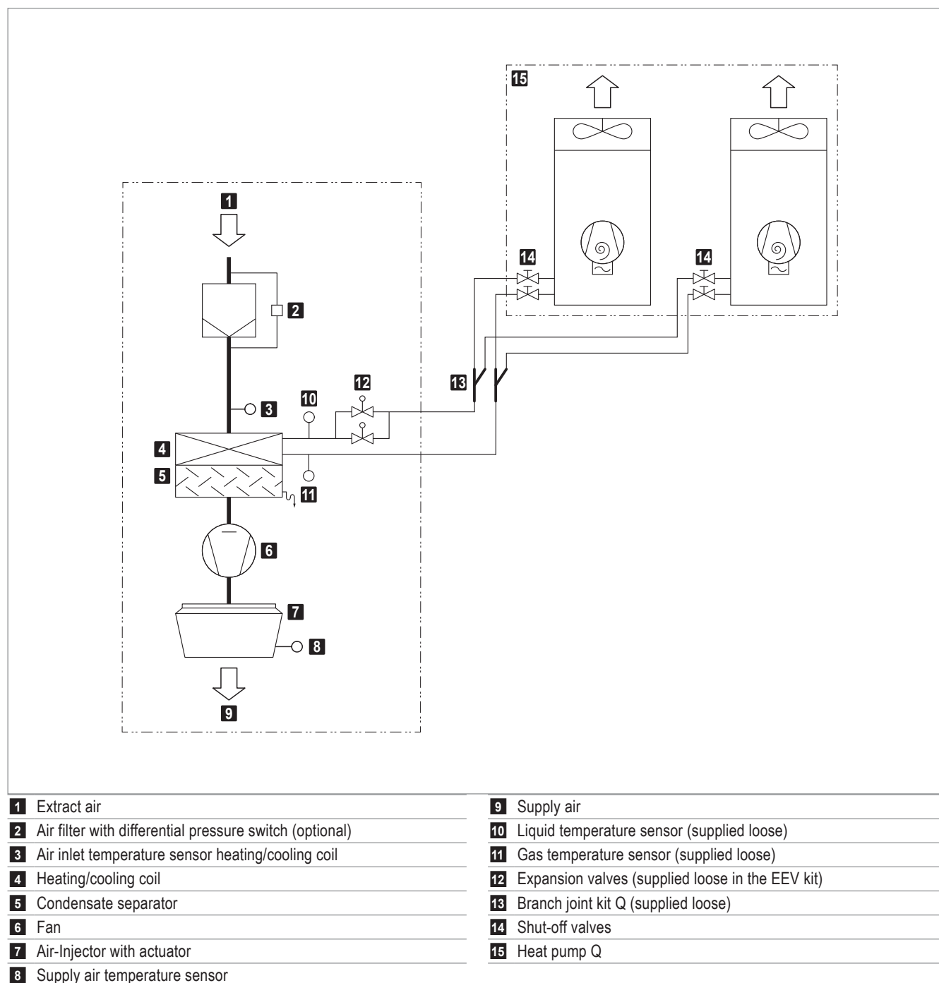
Fig. B4: TopVent® TP-9-Q function diagram
