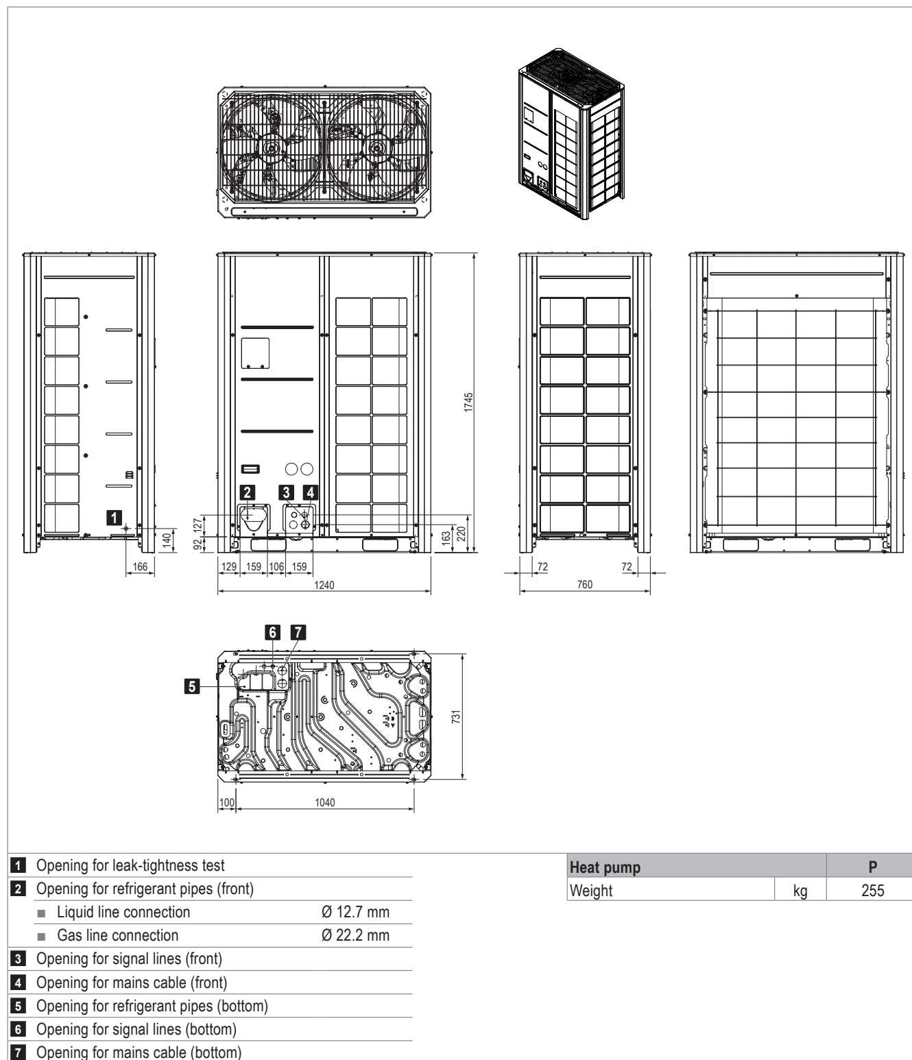
Fig. B7: Heat pump P dimensions and weights
