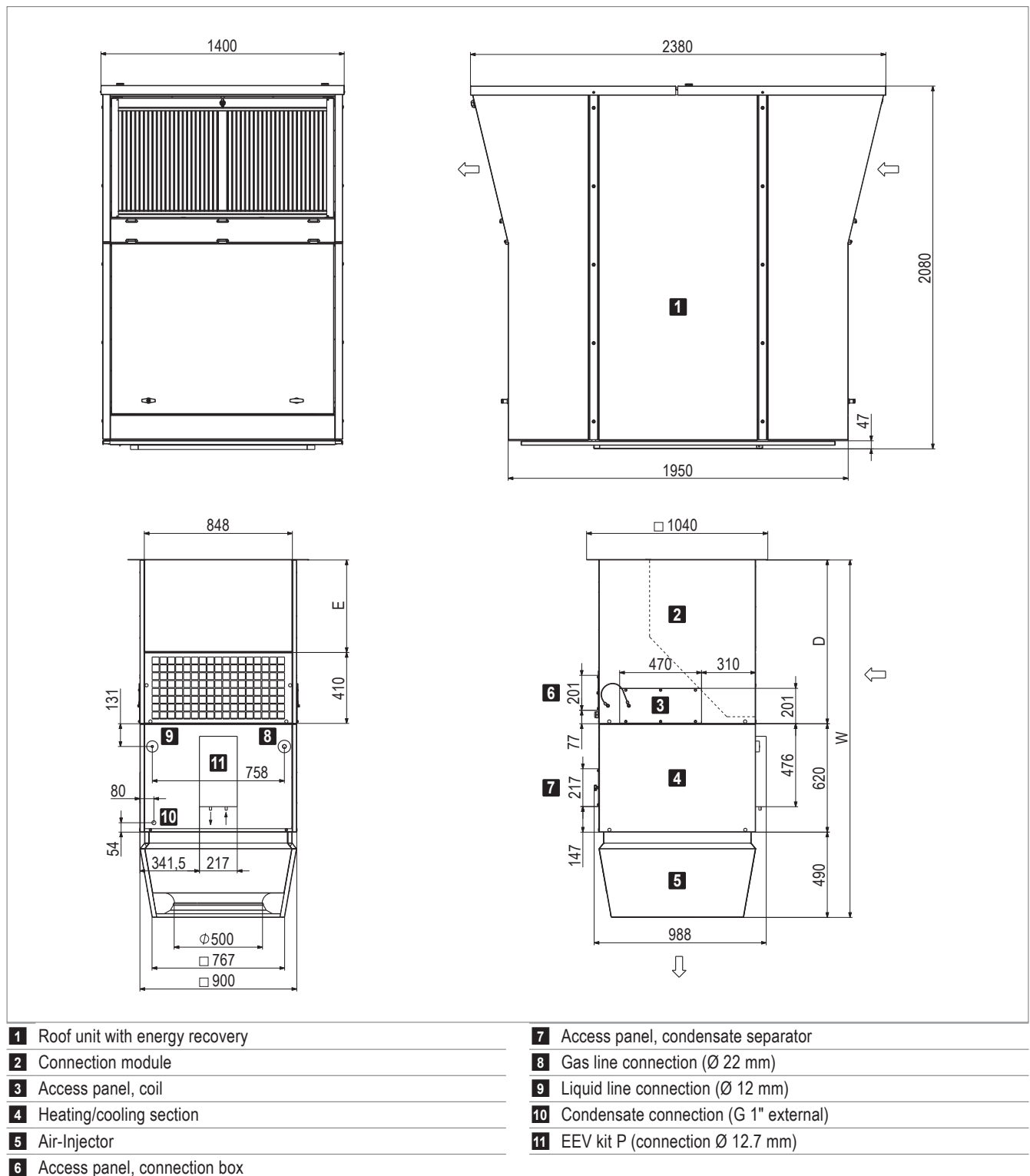
Fig. B4: RoofVent® RP-6-P dimensions
