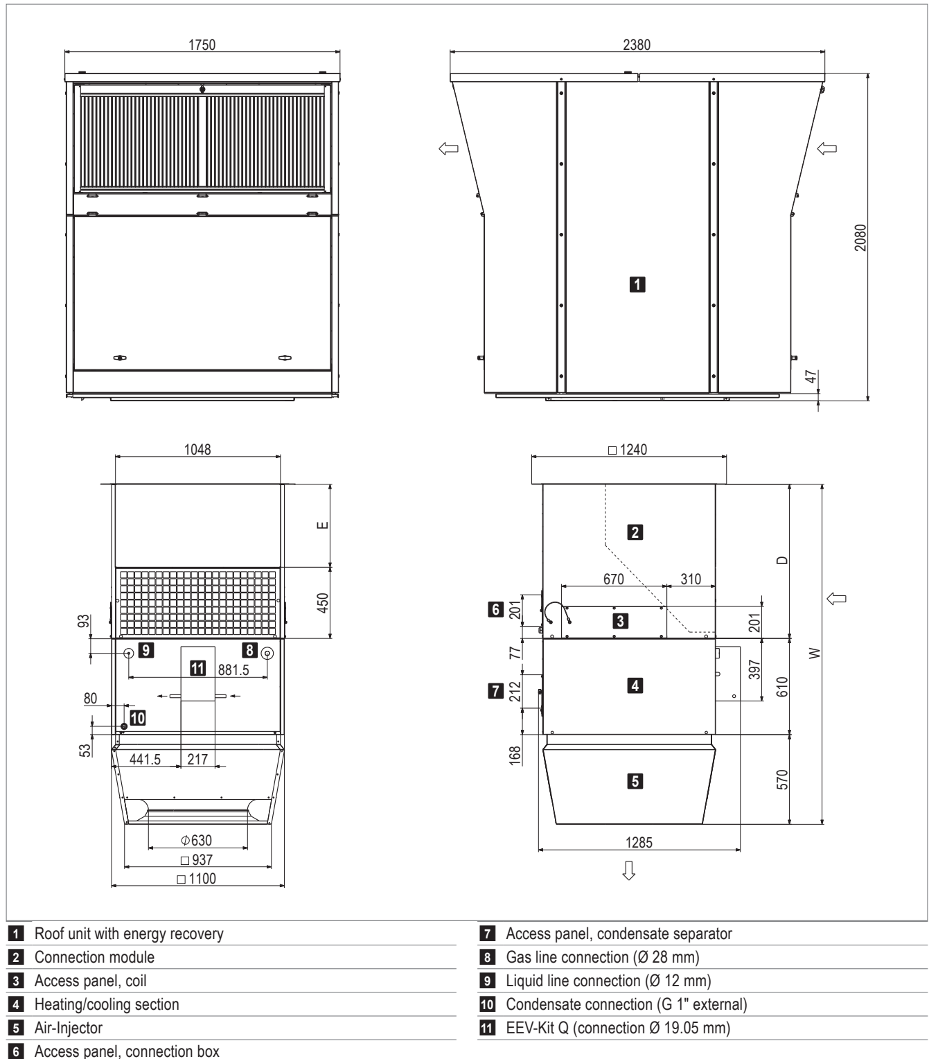
Fig. B6: RoofVent® RP-9-Q dimensions
