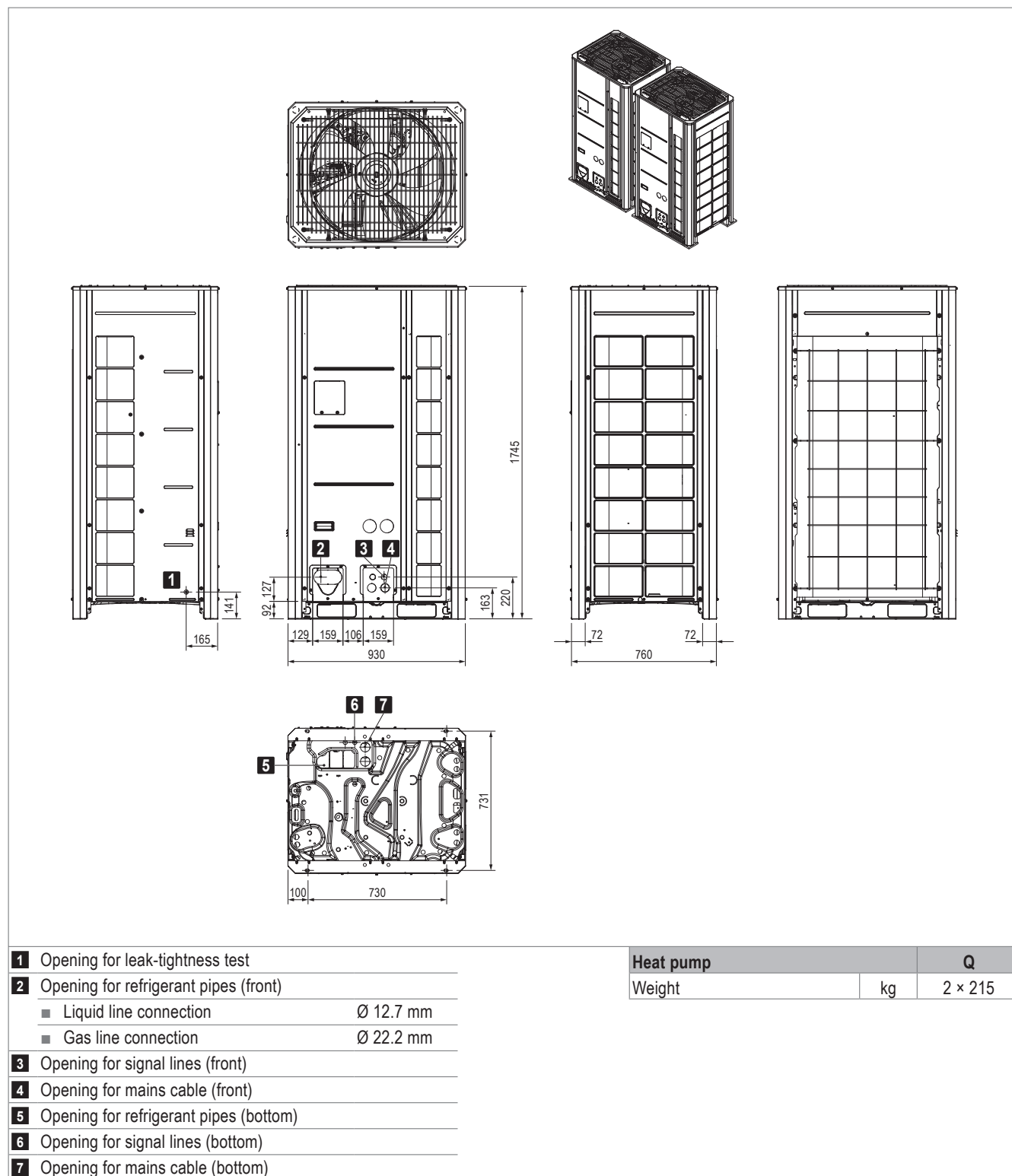
Fig. B8: Heat pump Q dimensions and weights
