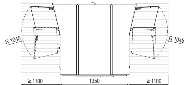
Fig. D2: Space requirements for maintenance on the roof (dimensions in mm)
