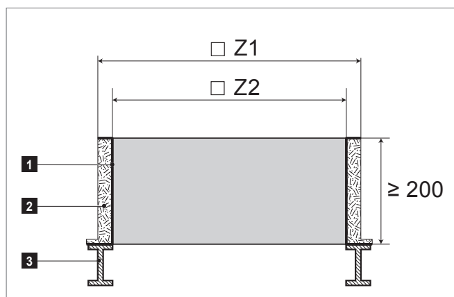
Fig. D8: Installation of RoofVent® units in the roof frame (dimensions in mm)
