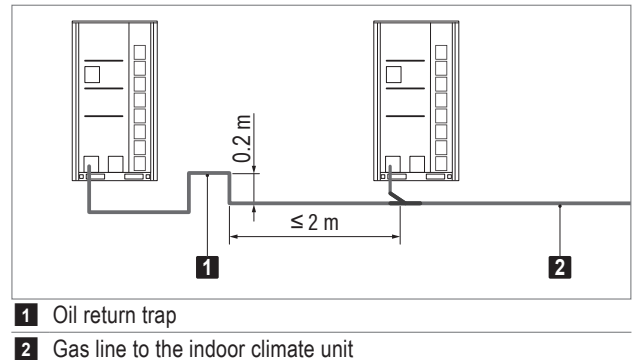
Fig. D17: Oil return trap
